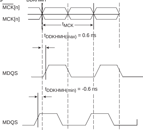
Figure 6-1. Timing Diagram for t_{DDKHMH}
